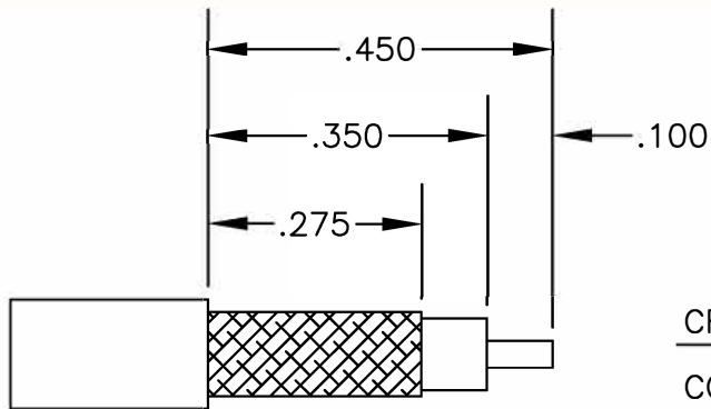
STRIPPING DIMENSIONS
