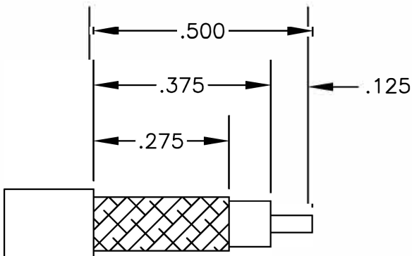
STRIPPING DIMENSIONS
