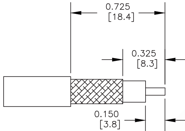
STRIPPING DIMENSIONS
