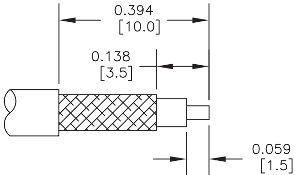
STRIPPING DIMENSIONS
