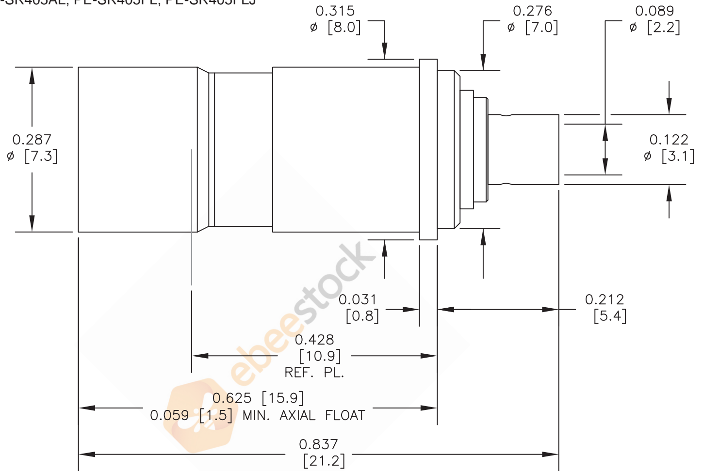
STRIPPING DIMENSIONS
