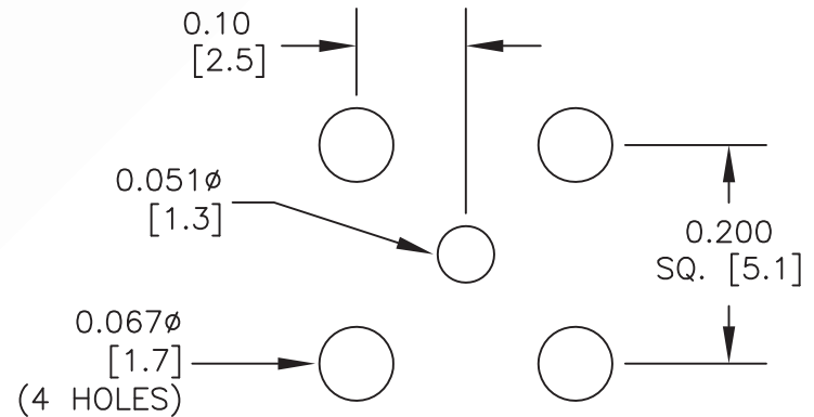
MOUNTING HOLES
