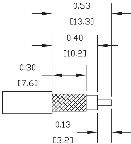
STRIPPING DIMENSIONS
