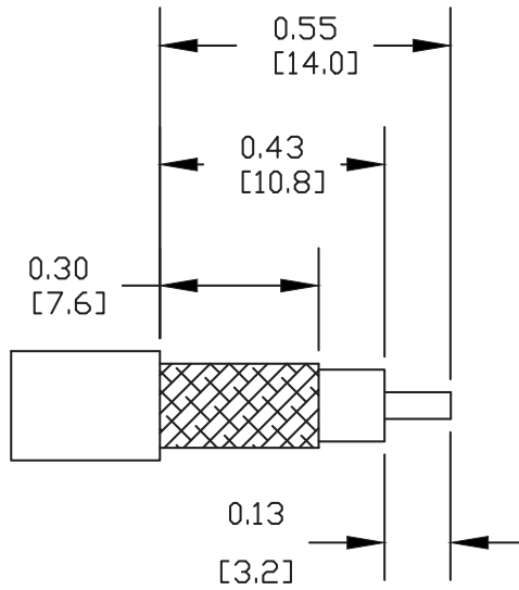
STRIPPING DIMENSIONS
