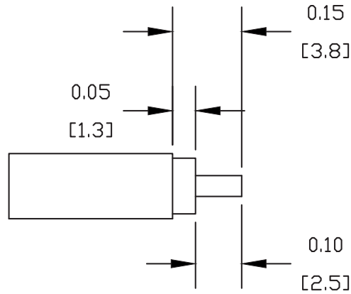
STRIPPING DIMENSIONS
