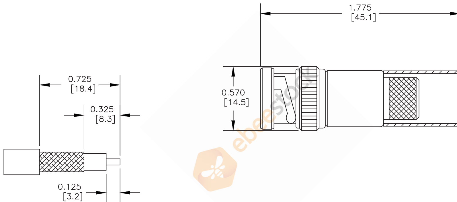
STRIPPING DIMENSIONS
