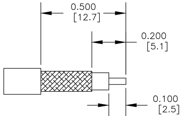
STRIPPING DIMENSIONS
