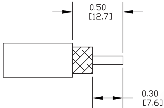
STRIPPING DIMENSIONS
