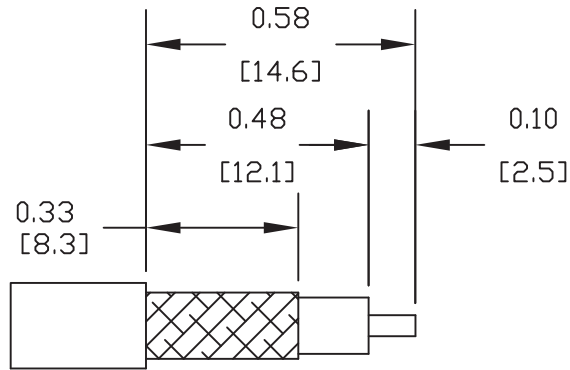
STRIPPING DIMENSIONS
