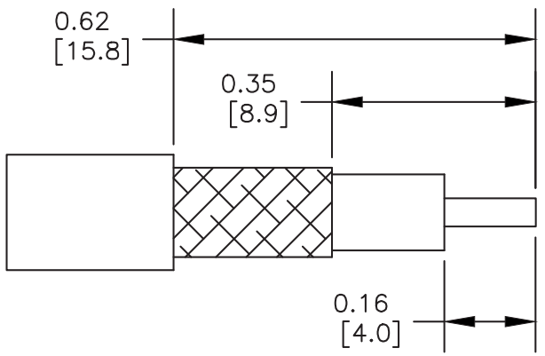
STRIPPING DIMENSIONS
