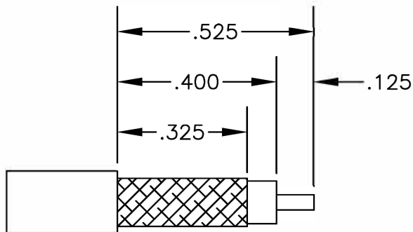
STRIPPING DIMENSIONS
