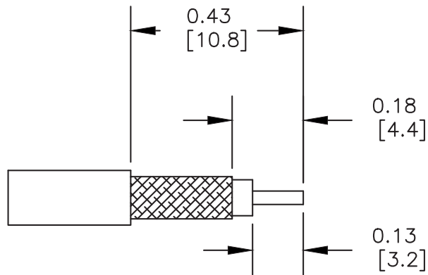
STRIPPING DIMENSIONS
