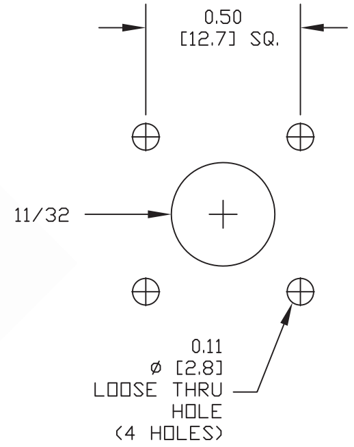
MOUNTING HOLES
