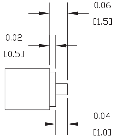
STRIPPING DIMENSIONS
