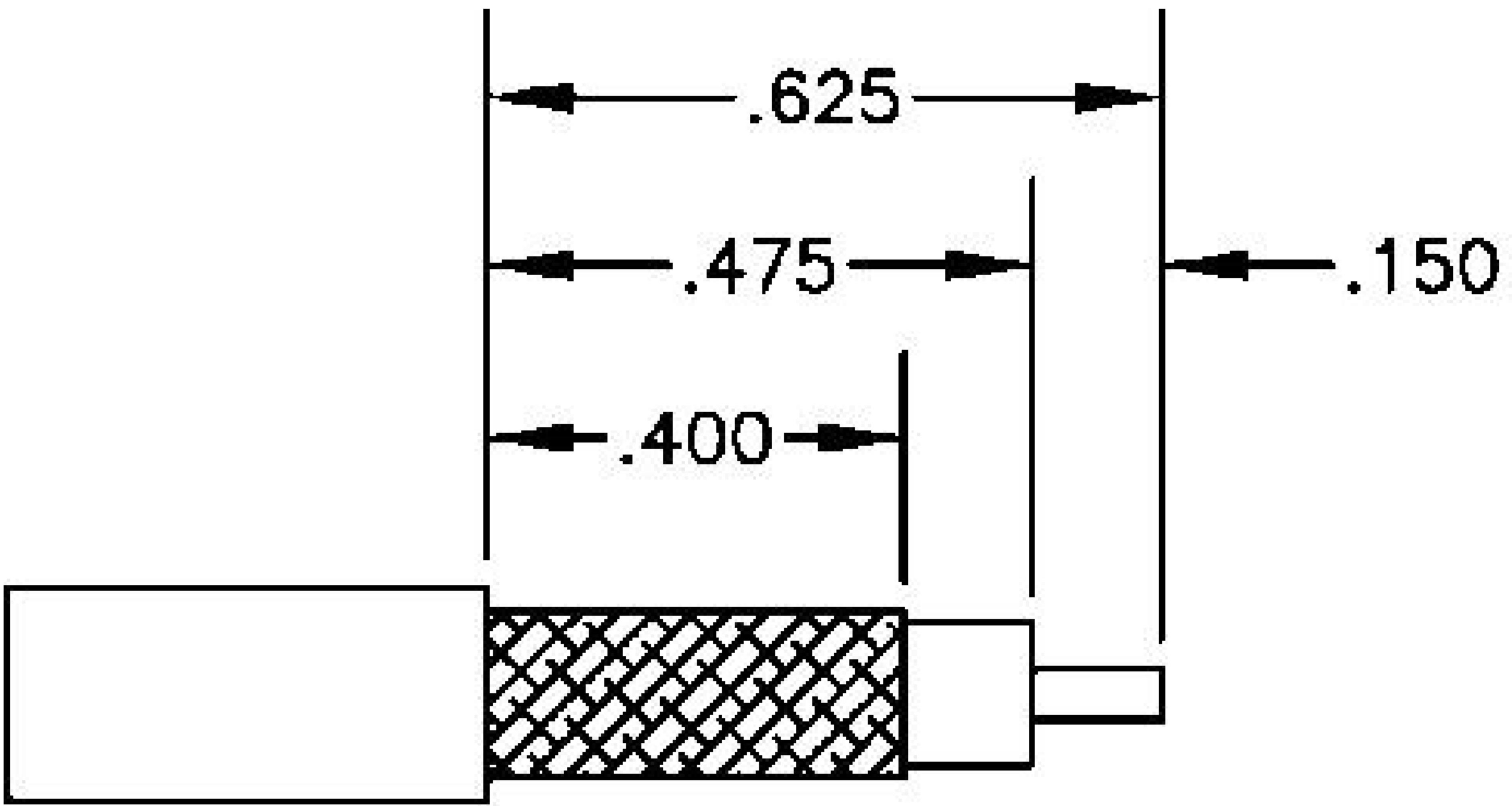
STRIPPING DIMENSIONS
