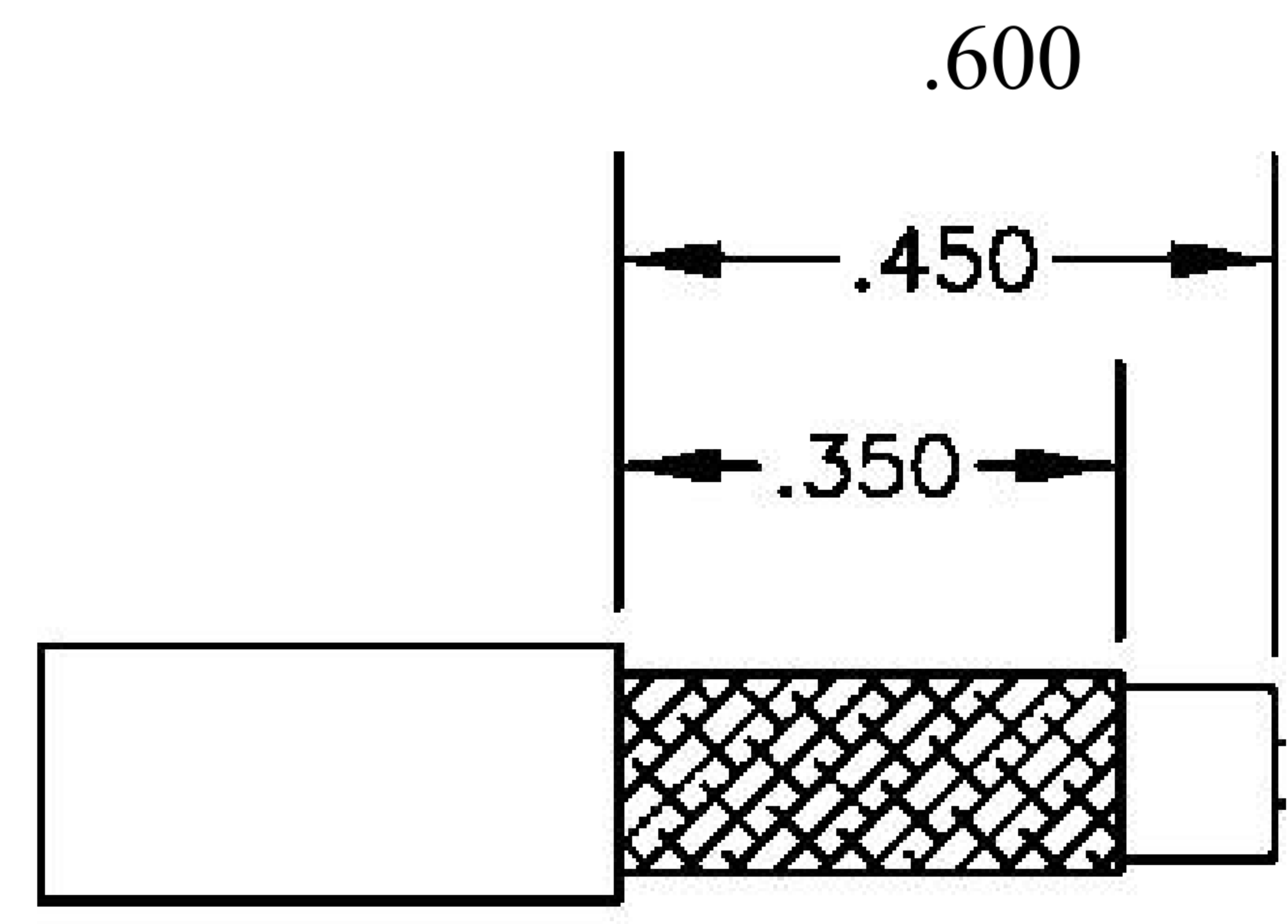
STRIPPING DIMENSIONS
