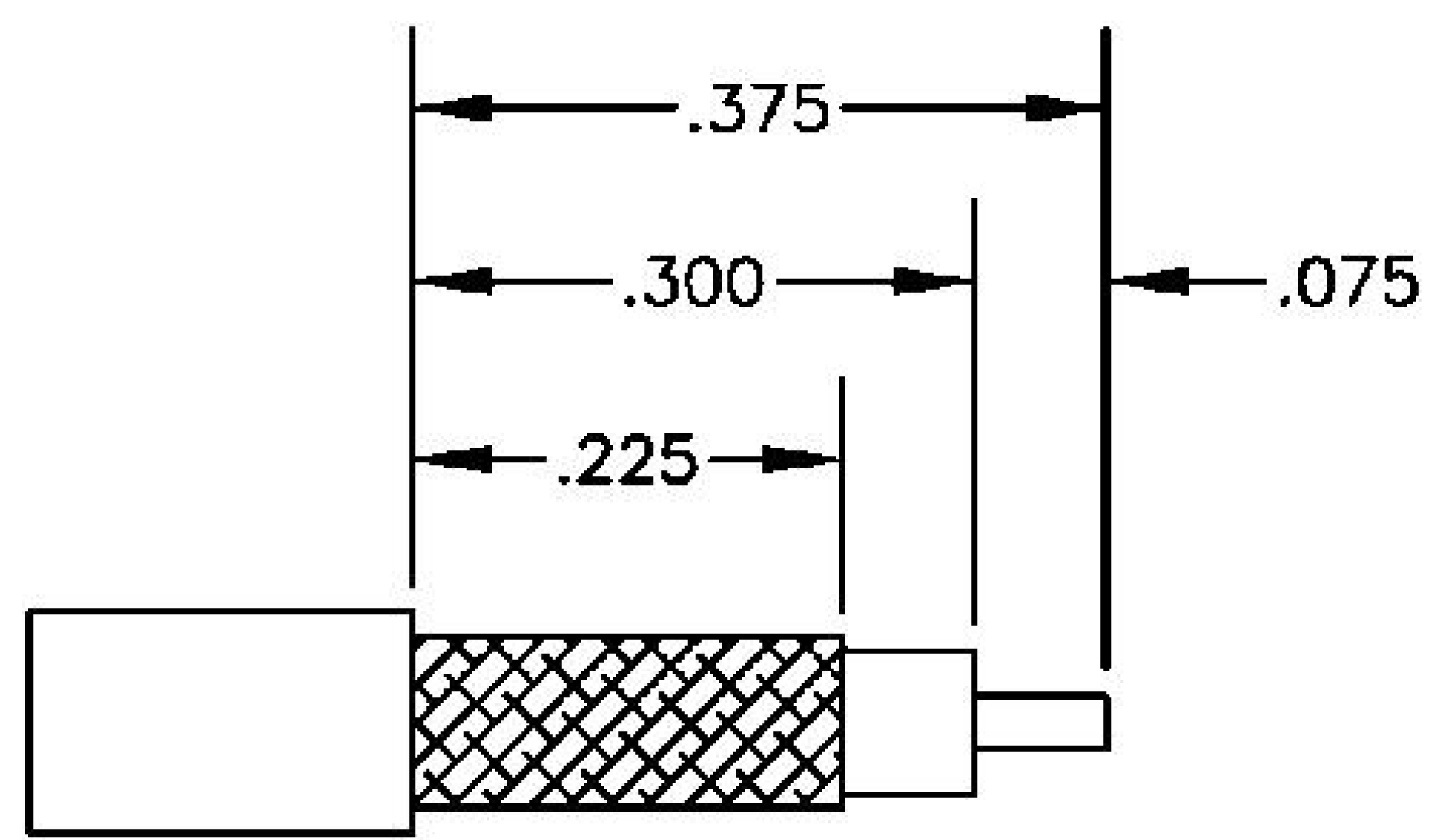
STRIPPING DIMENSIONS
