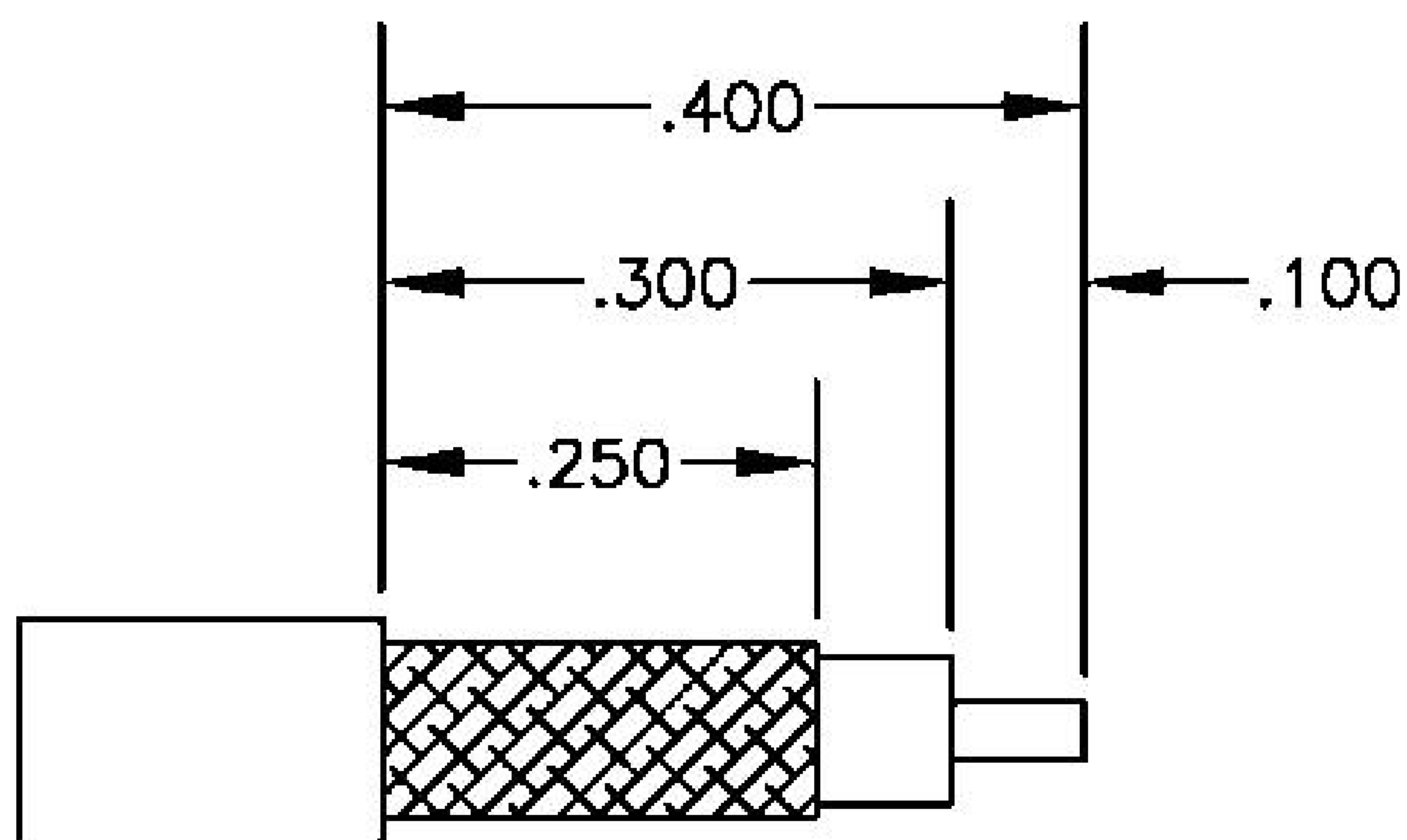
STRIPPING DIMENSIONS
