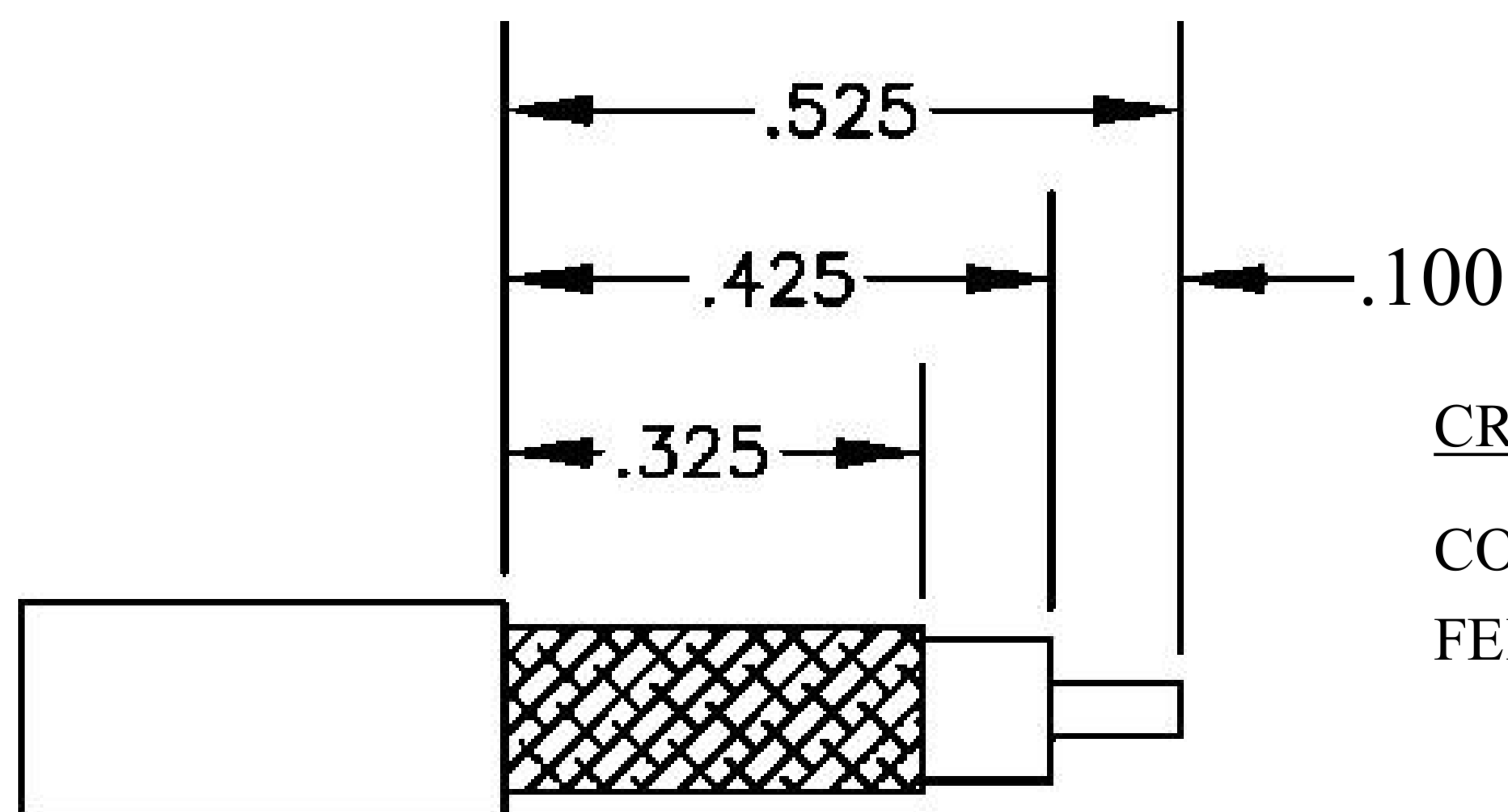
STRIPPING DIMENSIONS
