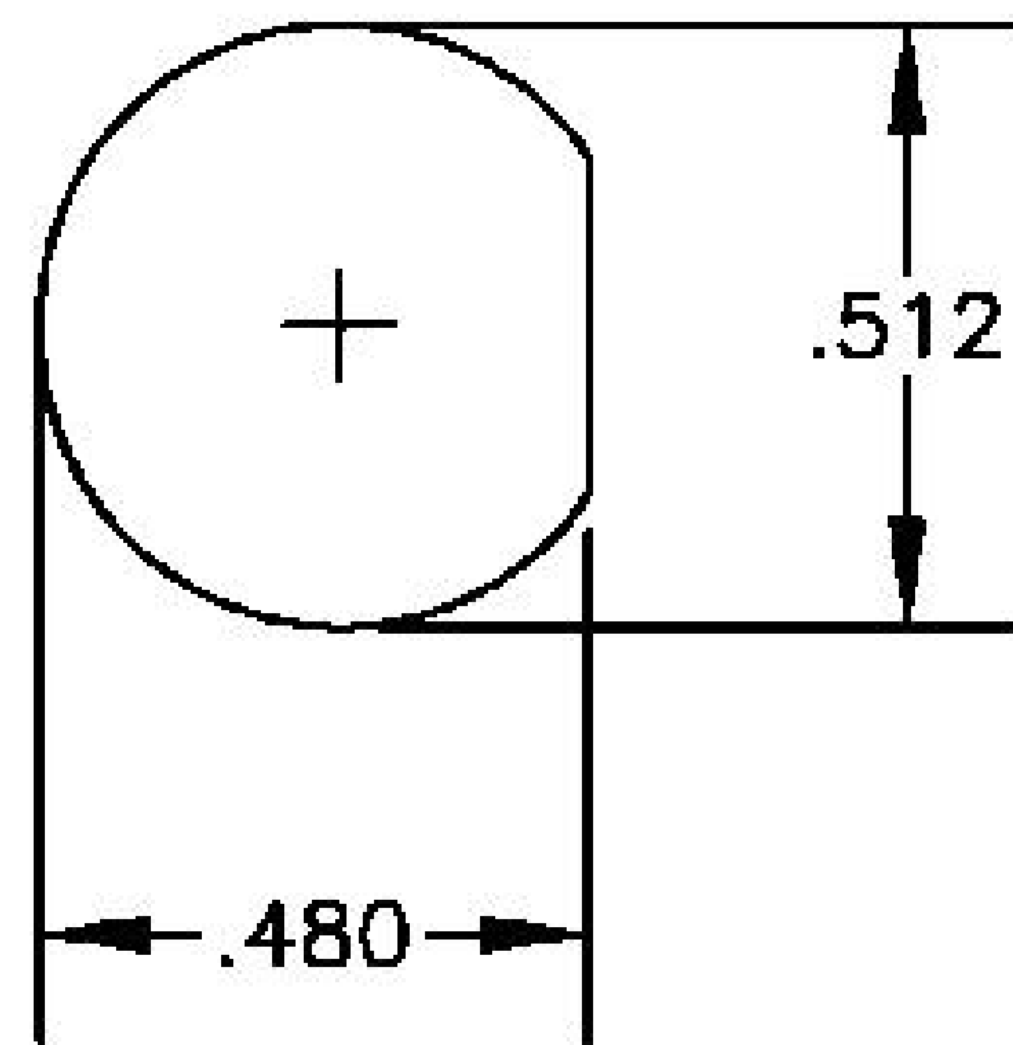
MOUNTING HOLE
