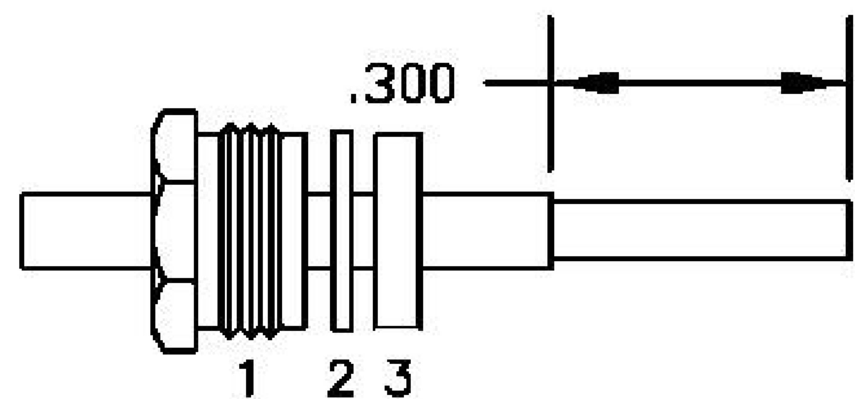
ASSEMBLY (A)
