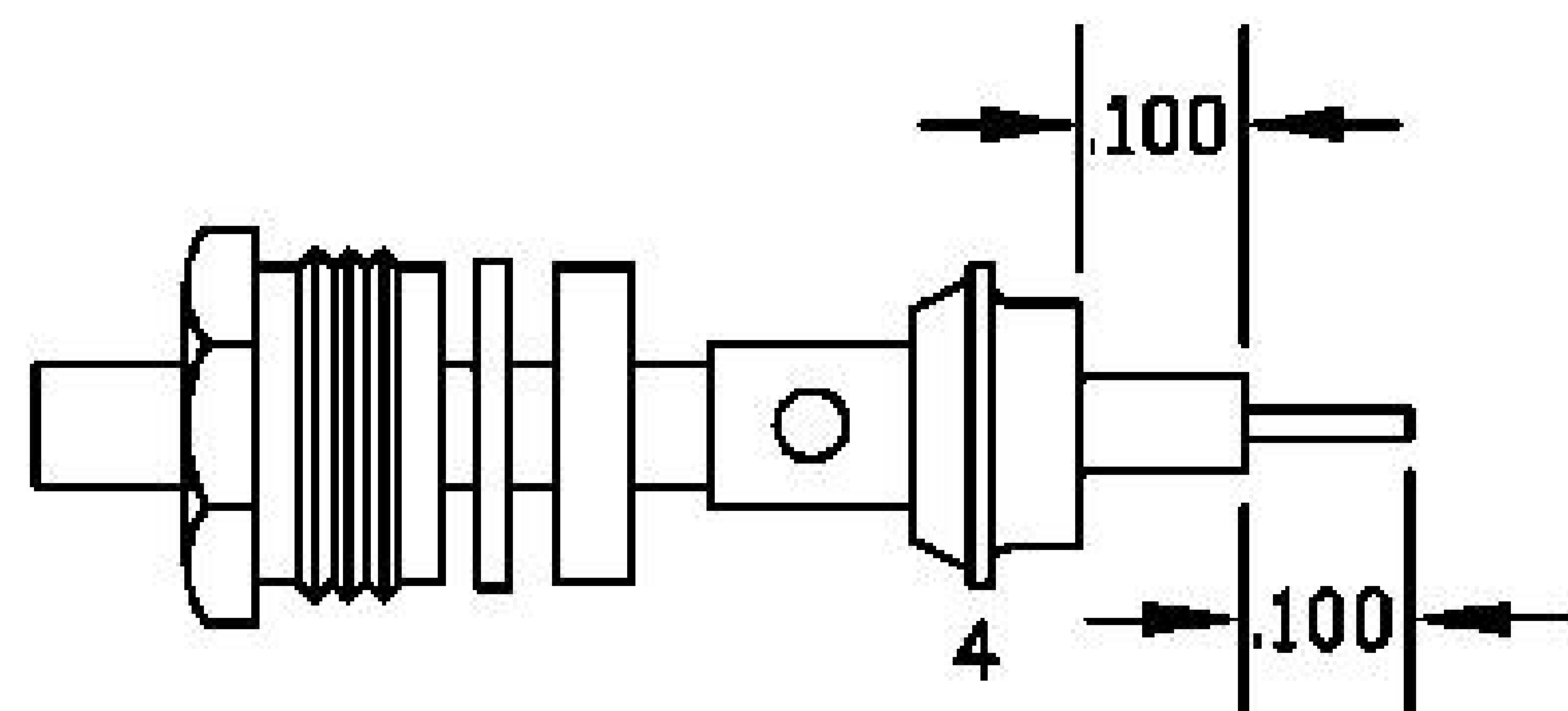
ASSEMBLY (B)
