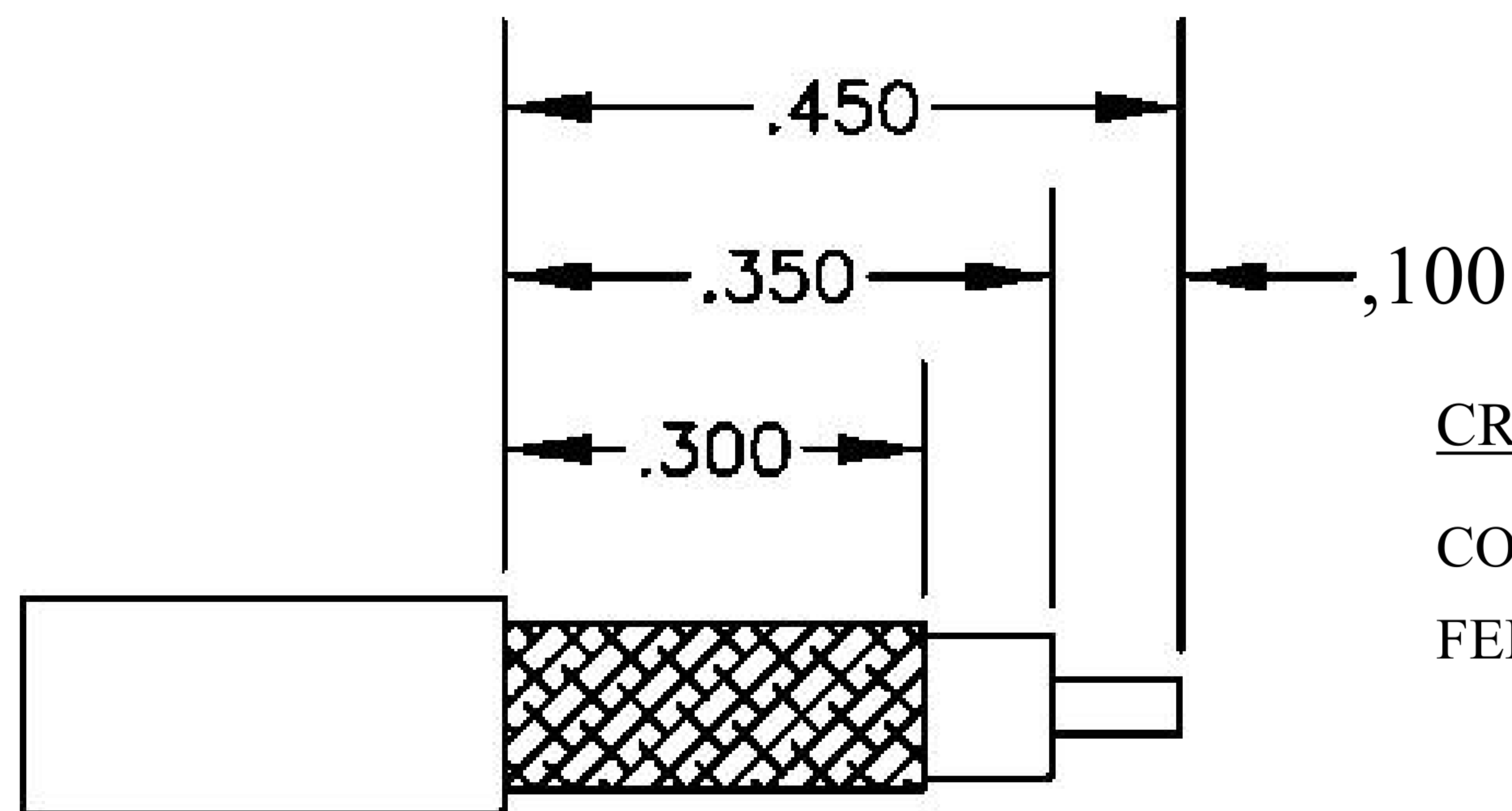
STRIPPING DIMENSIONS
